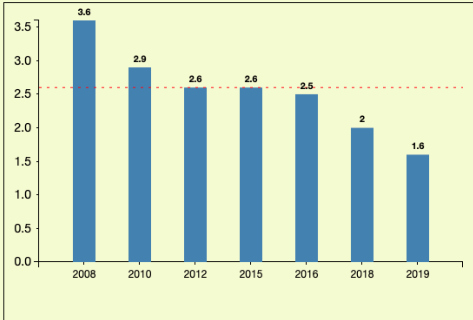
Concentration de chlorophylle a ( \mu\text{g/l} )
